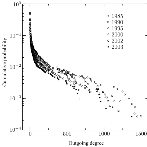
Figure 4.30. Change of degree distribution in a shareholding network.
