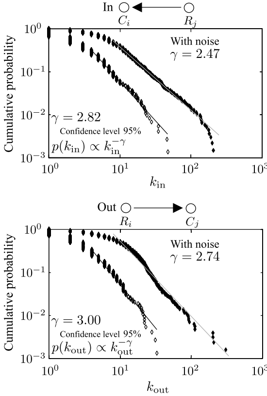
Figure 4.33. Cumulative probability distributions of incoming degree and outgoing degree.
