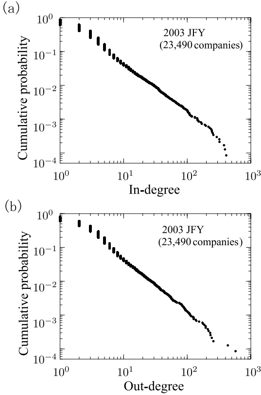
Figure 6.9. Cumulative distributions of (a) in-degree (vendors) (b) out-degree (customers).
