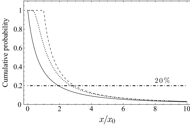
Figure 2.32. Various Pareto distributions and the 20% line.
