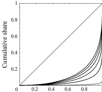
Figure 2.19. Lorenz curves for various values of \mu .
