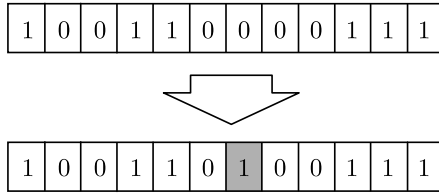
Figure 5.28. Mutation process.
