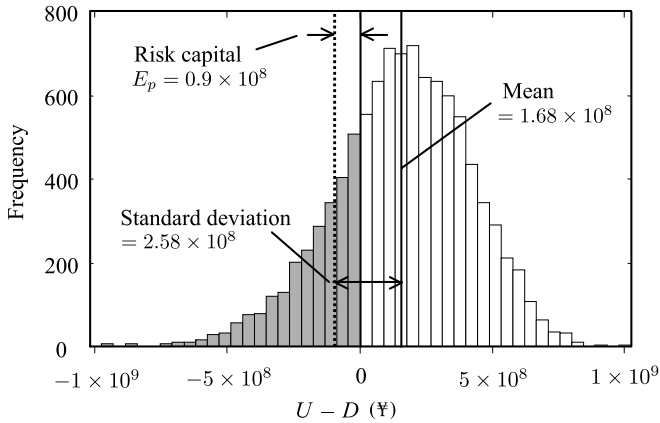
Figure 6.1. Distribution of U - D and risk capital E_p .
