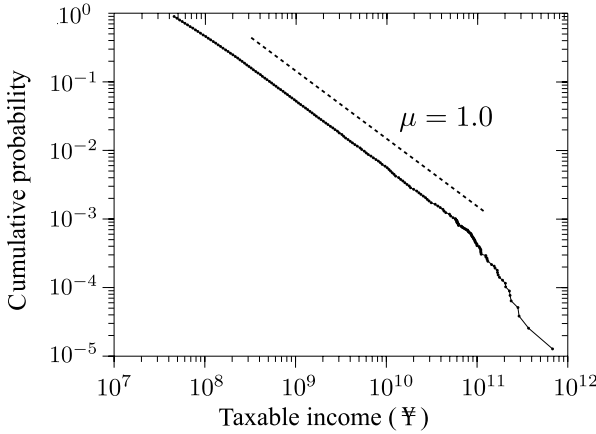
Figure 2.4. Double-logarithmic plot of CDF of companies' declared income.
