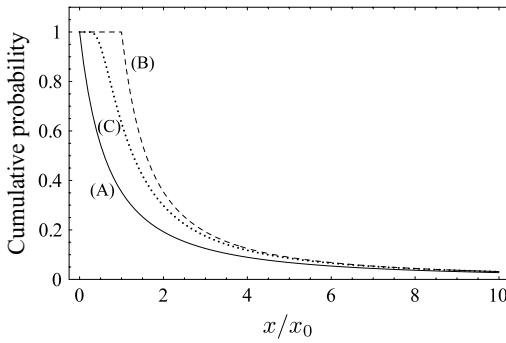
Figure 2.16. CDFs of various Pareto distributions.
