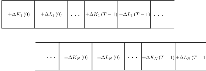
Figure 5.26. Gene.
