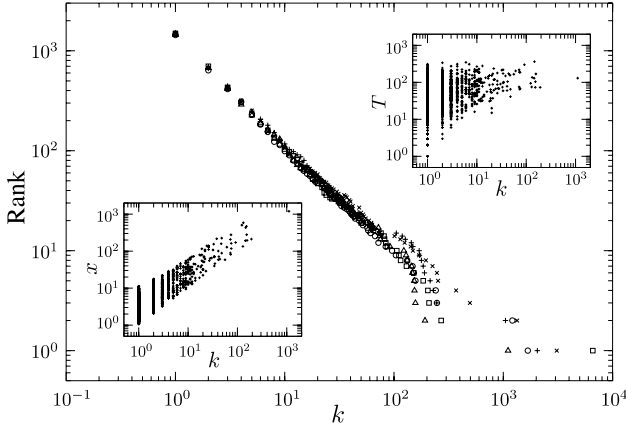
Figure 5.4. Conversion of the simulated results to the degree distribution.
