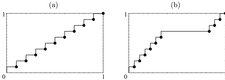
Figure 2.24. Examples of the staircase plot.
