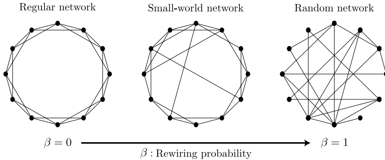
Figure 4.1. Watts–Strogatz \beta model.
