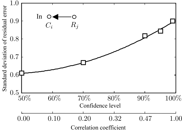
Figure 4.34. Standard deviation of residual error and confidence level.
