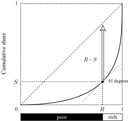
Figure 2.20. Definition of the Robin Hood index.
