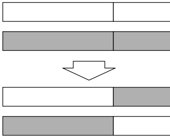
Figure 5.27. Crossover process.
