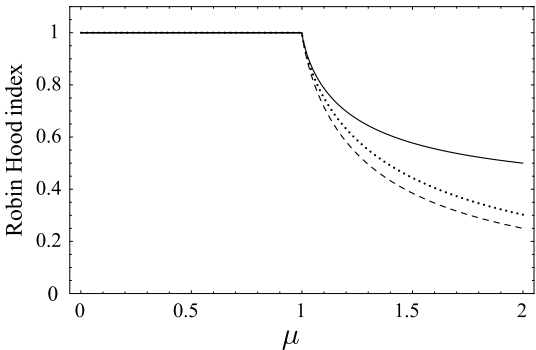
Figure 2.21. \mu -dependence of the Robin Hood index.
