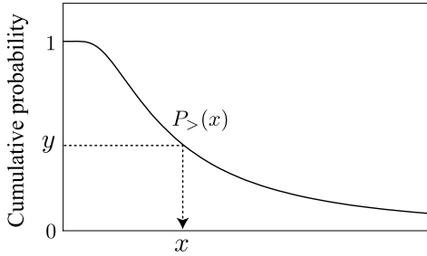
Figure 2.22. The inverse-function method to generate random numbers that obey an arbitrary distribution.
