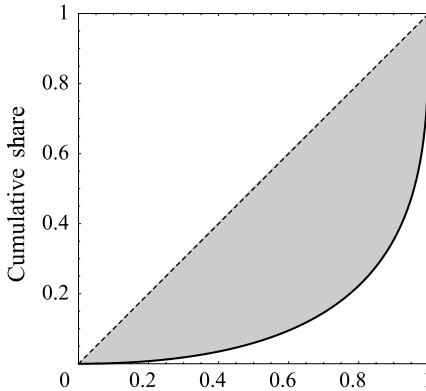
Figure 2.17. An example of a Lorenz curve.
