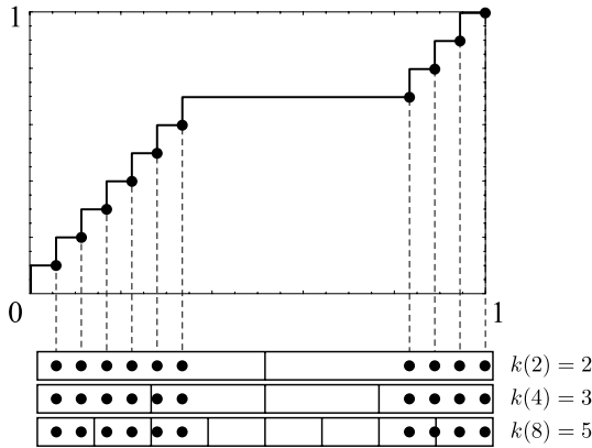
Figure 2.35. How to obtain the fractal dimension of the size distribution of companies.
