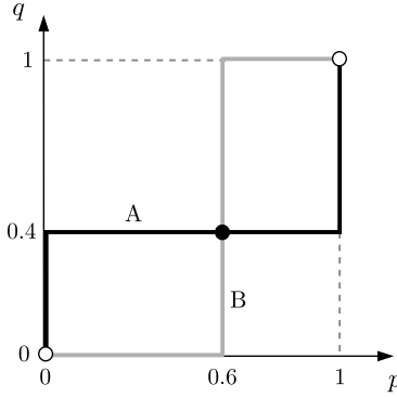
Figure 5.24. Multiple Nash equilibrium solutions.
