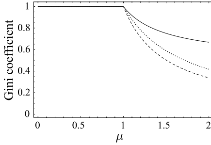
Figure 2.18. The \mu -dependence of the Gini coefficient.
