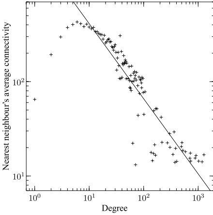
Figure 4.16. Degree correlation of the shareholding network.
