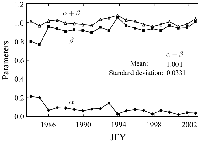
Figure 6.14. Parameters of the production function for companies belonging to a Japanese industrial group.
