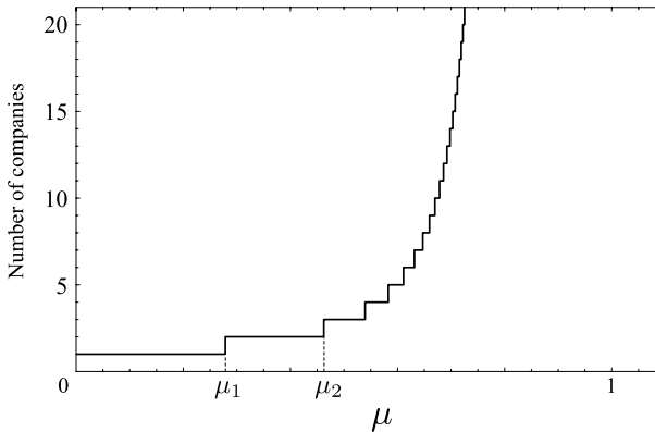
Figure 2.31. The minimum number, n , of the top n companies whose total share is greater than 80%.
