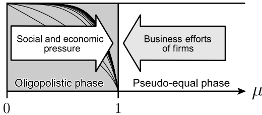
Figure 2.37. Two forces that besiege \mu = 1 .
