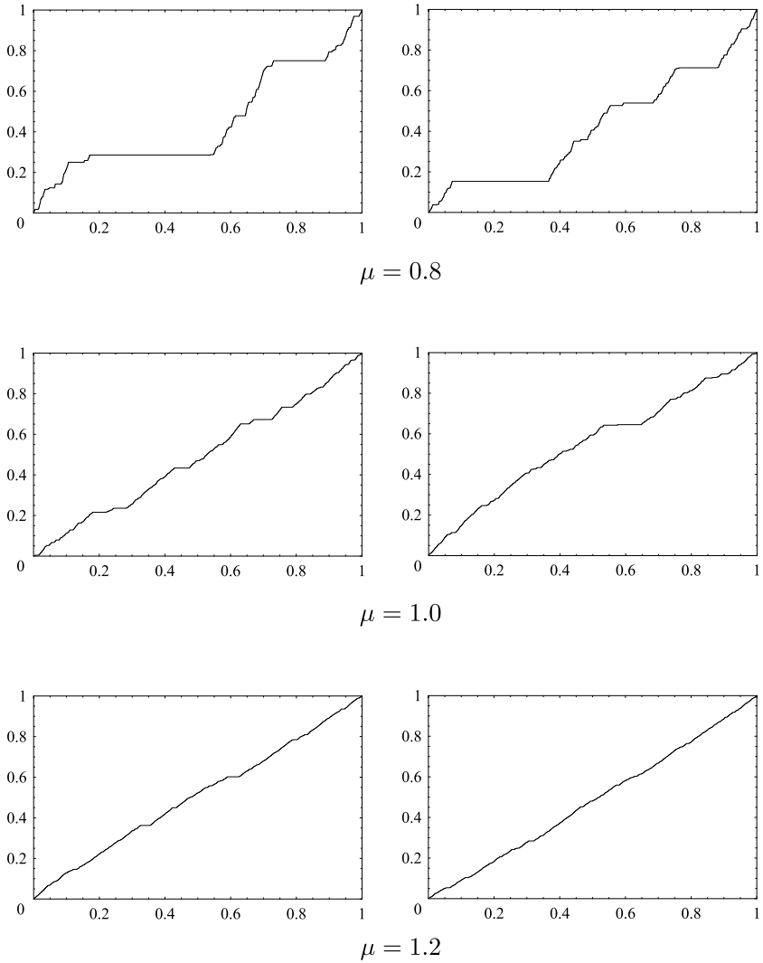
Figure 2.25. Devil's Staircases for \mu = 0.8, 1.0, 1.2 .
