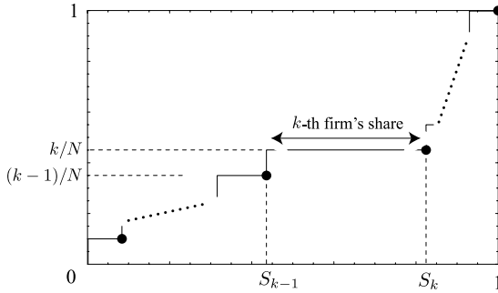
Figure 2.23. How to make a staircase plot. Each dot corresponds to a company.
