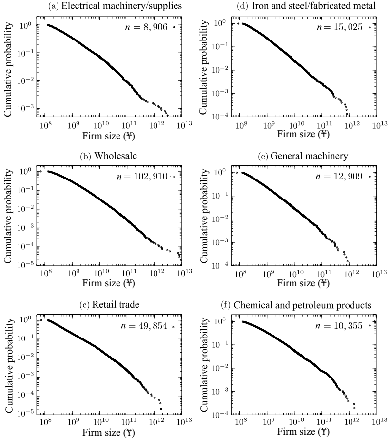
Figure 2.10. CDF of sales in various business sectors, 2002.
