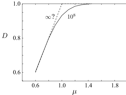
Figure 2.36. Fractal dimension of the Devil's Staircase.
